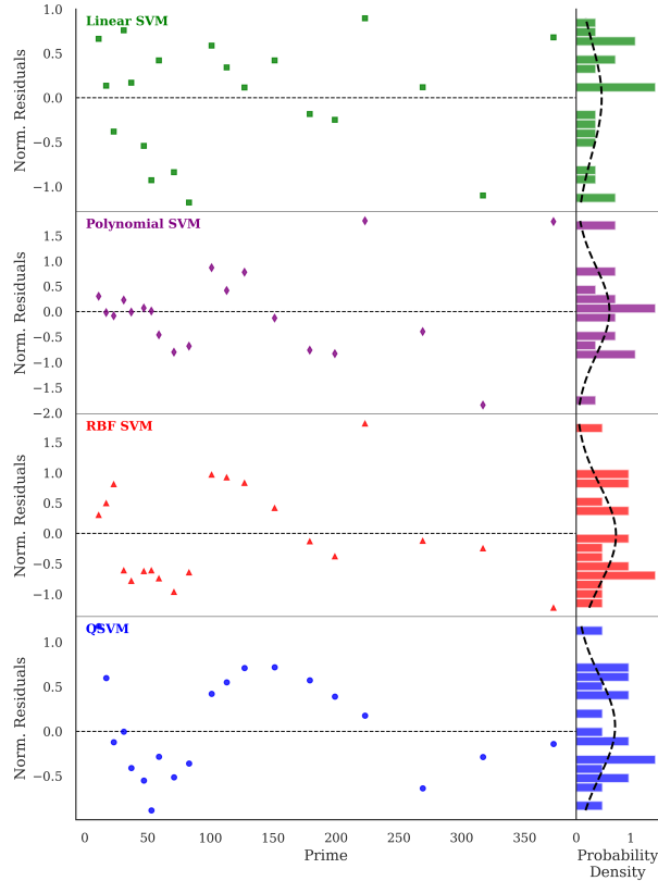
FIG. 10: Residual distributions for the logistic fit to the accuracy data. The QSVM residuals (blue) exhibit a pronounced periodic trend and lower overall variance compared to the classical SVM models.
