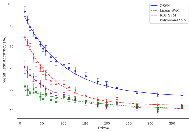
FIG. 5: Accuracy as a function of prime size for each model, overlaid with a 4-parameter logistic fit.
