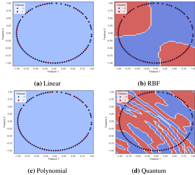
FIG. 6: Comparison of decision boundaries for each kernel illustrating how the models divide the feature space for an example dataset ( p = 101 ).
