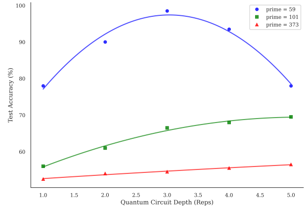
FIG. 7: QSVM accuracy as a function of circuit depth for varying dataset complexities controlled by prime size.
